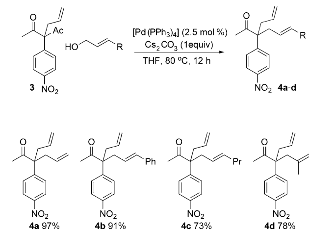
Scheme 3. Deacylative allylation of an acetyl acetone derivative.
